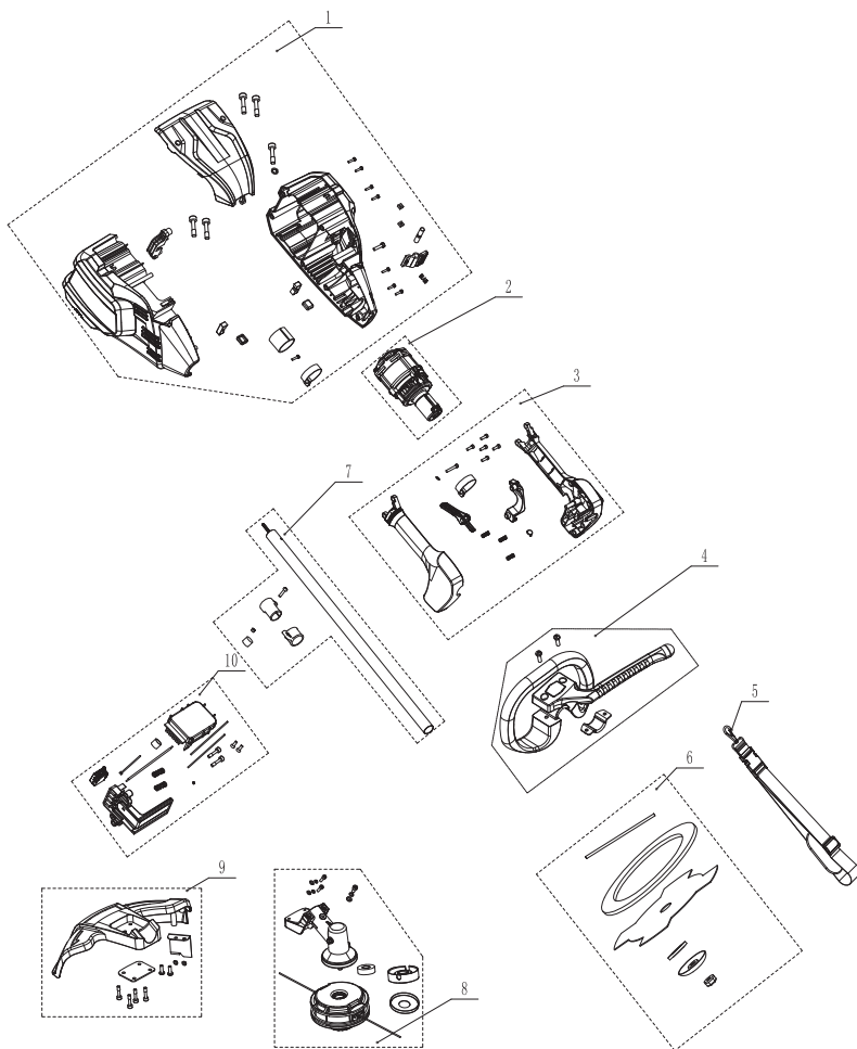
String Trimmer, PC82ST, 2100313
