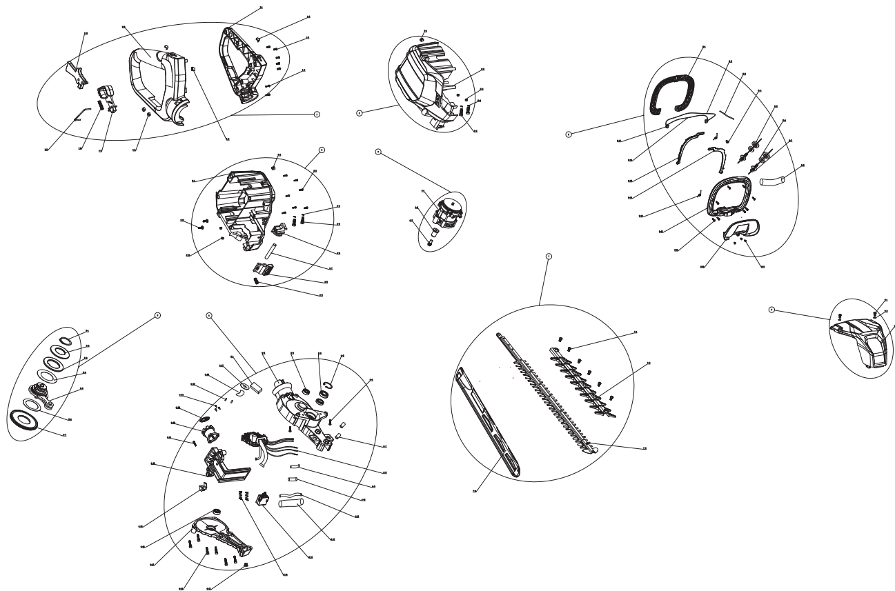
Hedge Trimmer, PC82HT, 2200413
