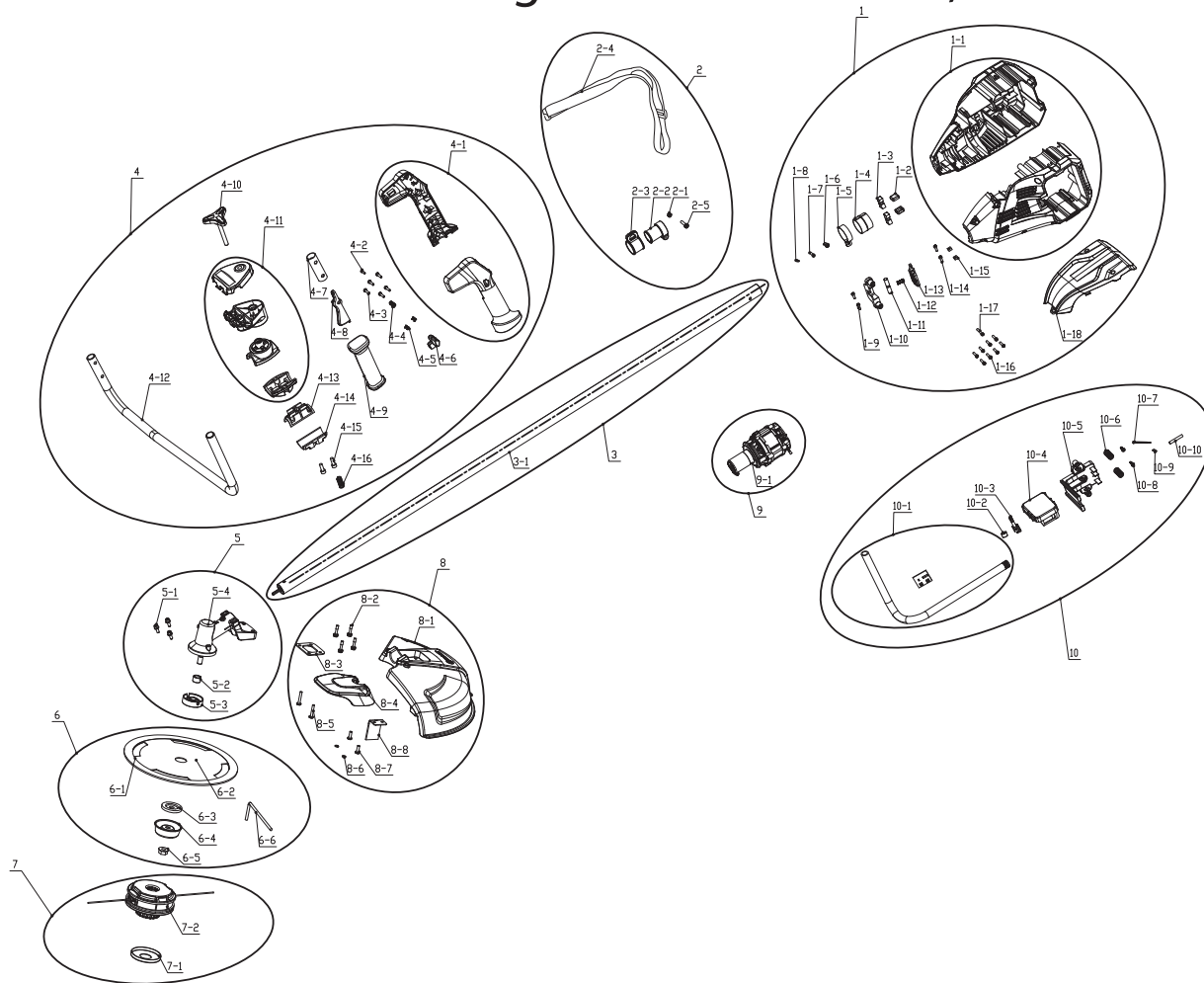
String trimmer PC82BC, 2100413
