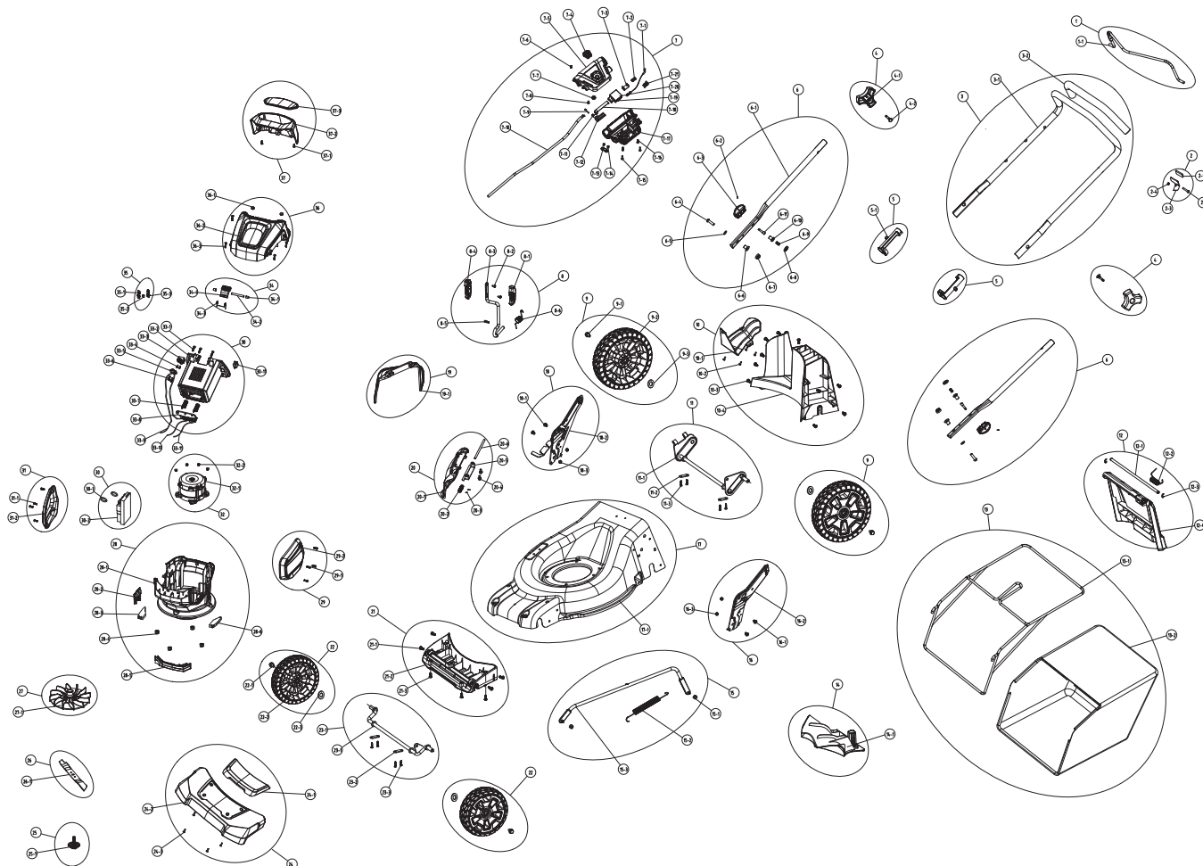
Lawn Mower PC82LM46, 2500813
